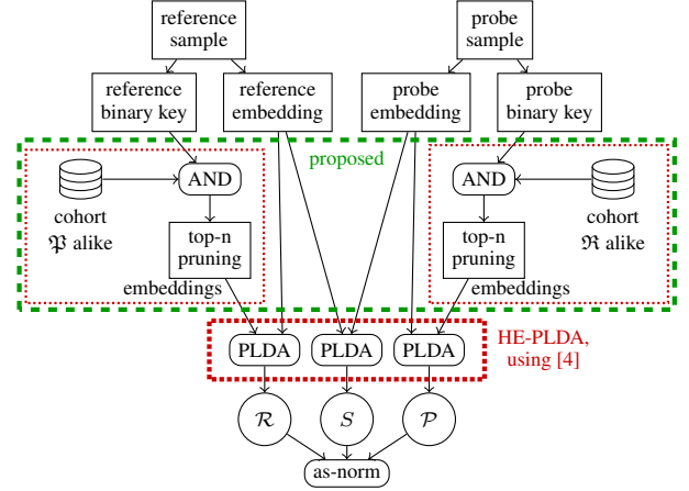
Figure 2: Our proposed privacy-preserving as-norm protocol with cohort pruning (green dashed area). The red dotted areas indicate that operations are carried out in the encrypted domain and do not leak any information except the decryptable outputs.
