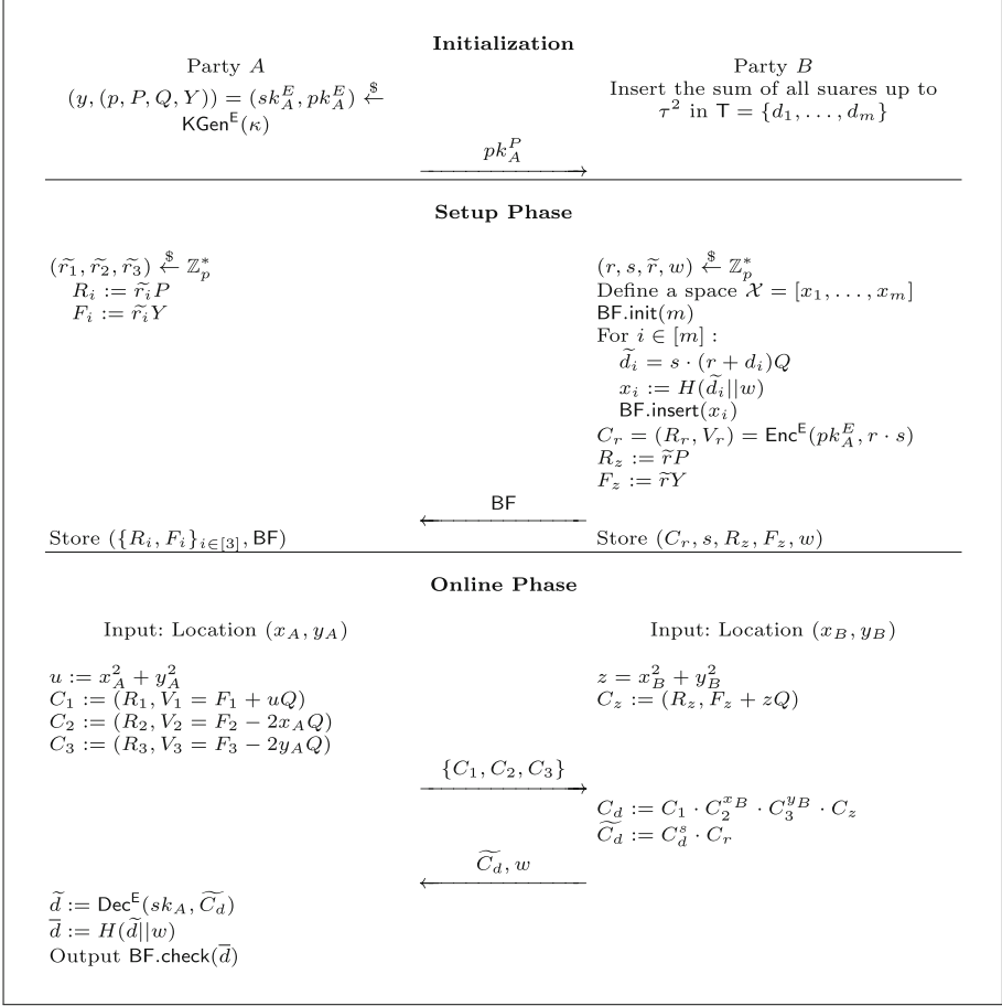
Fig. 4. Our PPLP protocol \Sigma_{\text{EIG}} using ElGamal encryption.
