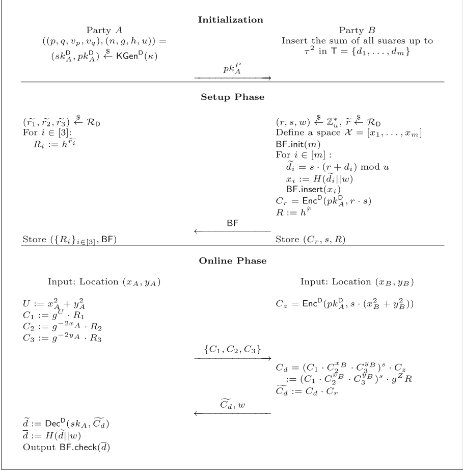
Fig. 3. Our PPLP protocol \Sigma_{\text{DGK}} using DGK encryption.
