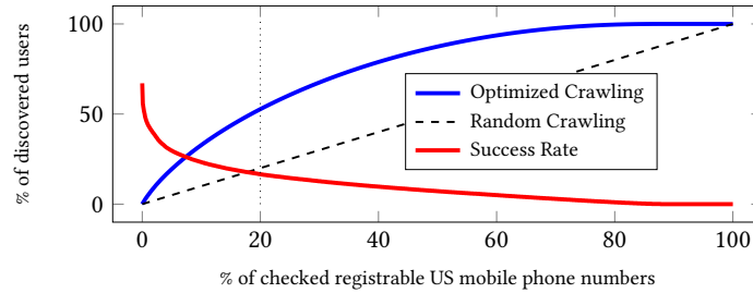
Fig. 3. Optimized crawling compared to random crawling based on the non-uniform distribution of registered WhatsApp users across the US mobile phone number space.
