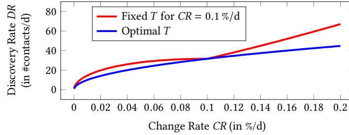
Fig. 5. Minimal discovery rate for different change rates CR with optimal choices for T (for Signal’s parameters) compared to the discovery rate for fixed T when estimating CR = 0.1\%/d .
