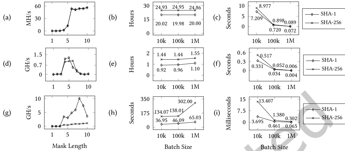
Fig. 2. Brute-force benchmark results for masked hashcat (a–c), hybrid hashcat (d–f), and hybrid JTR (g–i).
