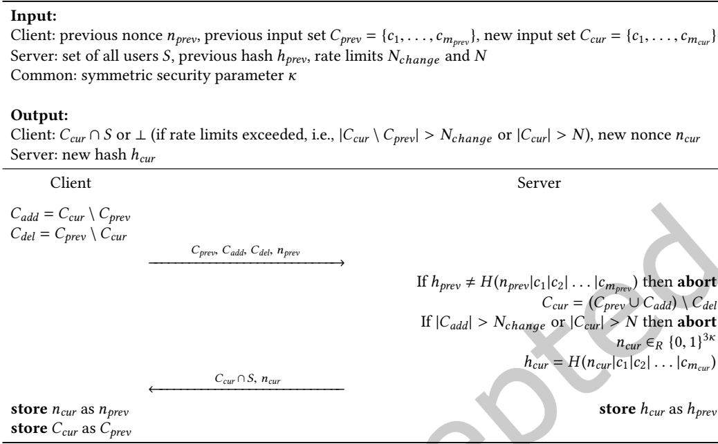
Fig. 6. Differential contact discovery.
