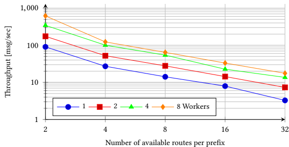
Figure 11: Throughput test of SIXPACK for different number of parallel workers.
