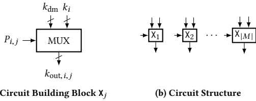
Figure 6: The EXPORT-ALL circuit is a set of |M| multiplexers, each of which outputs either the valid or dummy key depending on entry P_{i,j} , where i ( j ) is the member announcing (receiving) a route.
