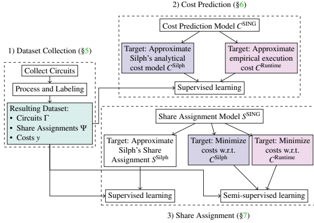
Figure 1: Overview of our SING framework and approach for ML-based MPC protocol assignment, consisting of MPC Dataset Collection (§5), MPC Cost Prediction (§6), and MPC Share Assignment (§7).
