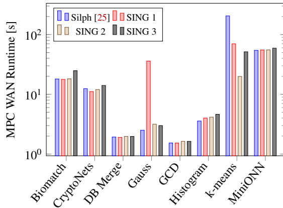
Figure 3: Comparison of resulting MPC WAN runtimes (s) for different share assignments. Detailed results in Table 7.
