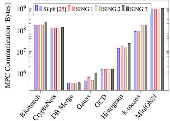
Figure 4: Resulting MPC communication (Bytes) for different share assignments; detailed results in Table 8.
