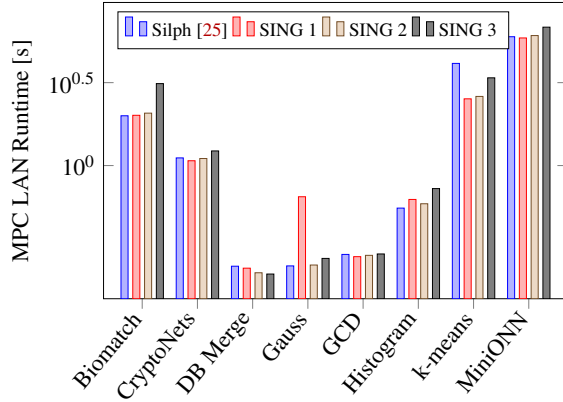
Figure 2: Comparison of resulting MPC LAN runtimes (s) for different share assignments. Detailed results in Table 6.
