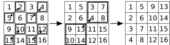
Figure 2: Efficient matrix transposition of a 4 \times 4 matrix using Eklundh’s algorithm.
